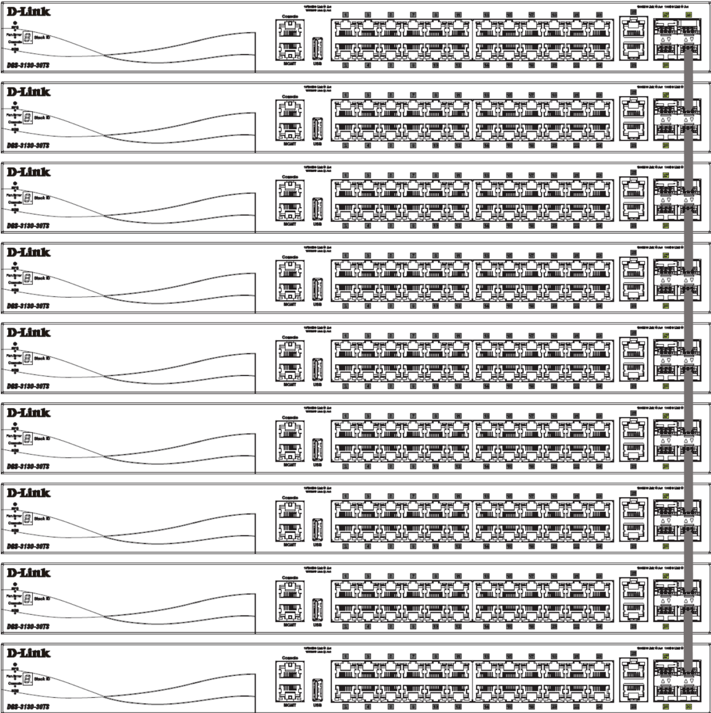
Figure 4-4 2-Port Duplex Chain stacking topology (SFP+ ports)
